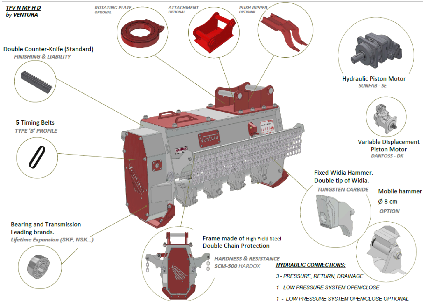
Reinforced mobile hammer double cutter
